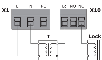
Figure 22. Connection diagram for an electromagnet lock
